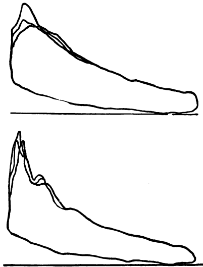
FIG. 133.—Typical Gas-Engine Indicator Cards, taken under actual service conditions. The first diagram is from an engine running under half load; the second from one "t full load. Both exhibit the variations in the expansion curve, usually attributed to consecutive explosions. These cards are composites of three successive strokes each.
